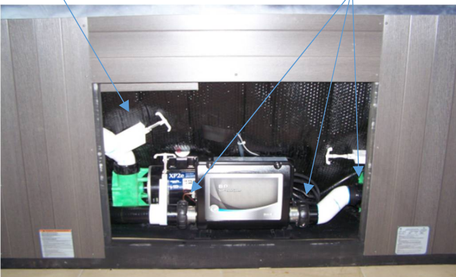
GATE VALVE
